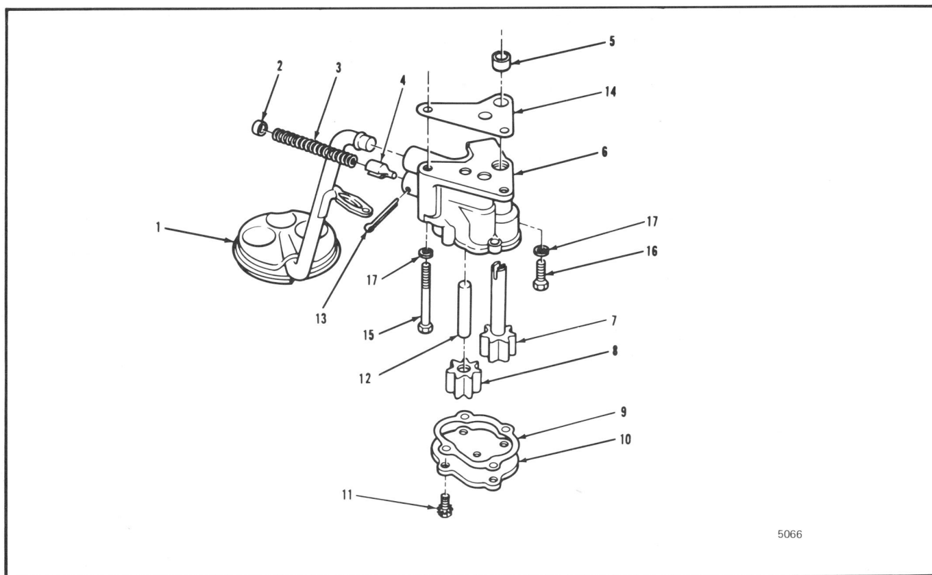
Figure 1-8 Oil Pump
