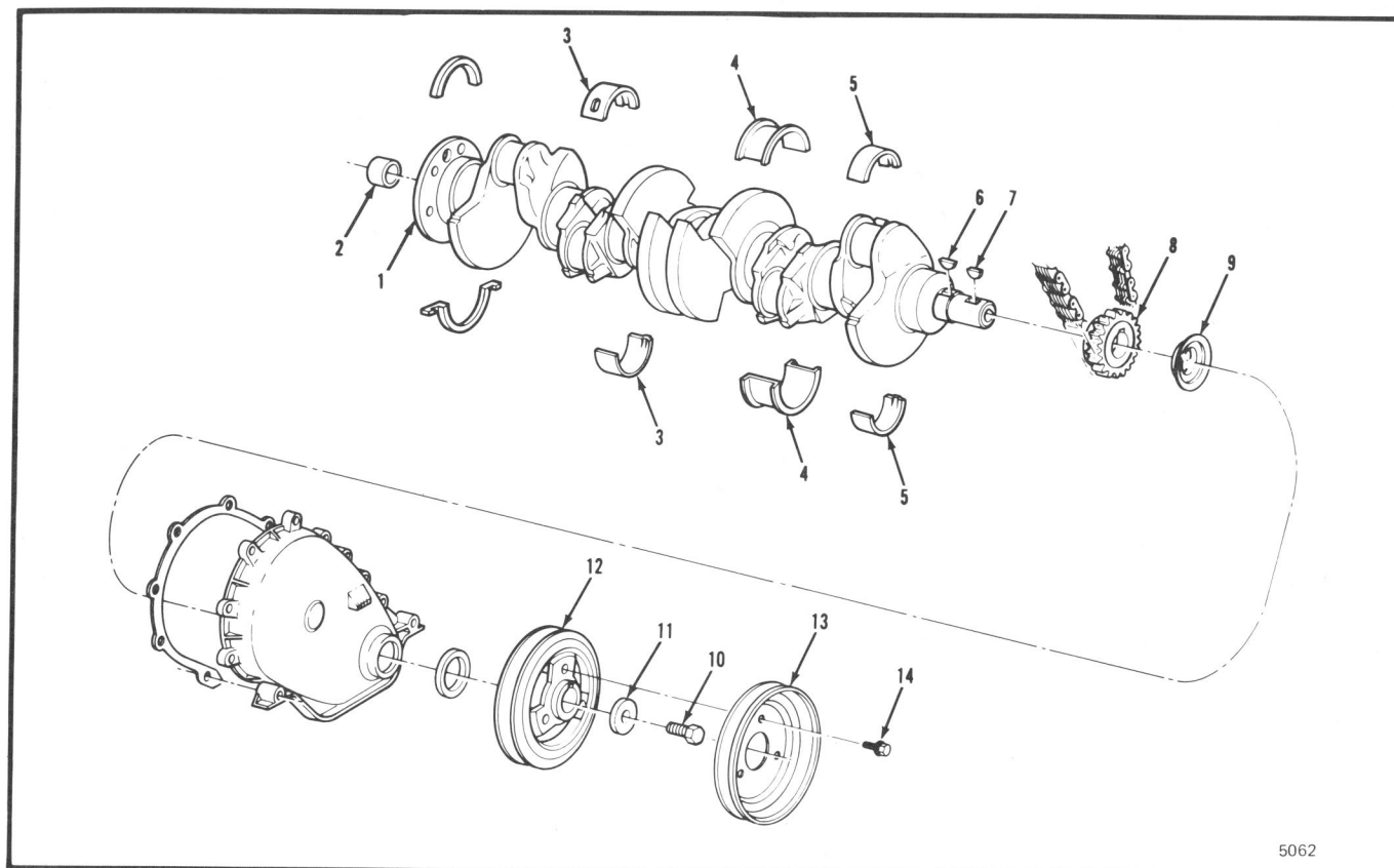
Figure 1-3 Crankshaft Vibration Damper and Main Bearings
