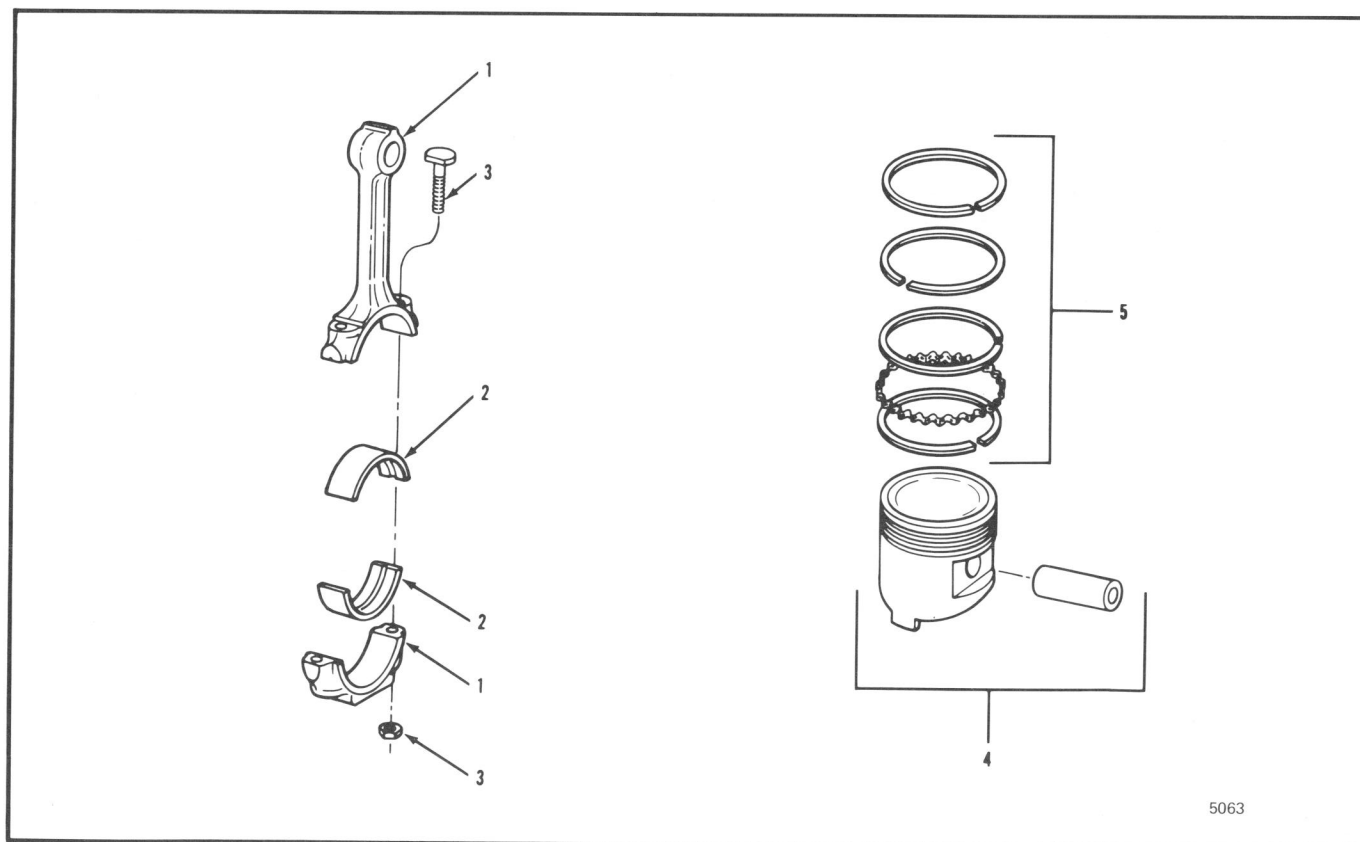
Figure 1-4 Connecting Rods and Bearings, Pistons, Pins and Rings
