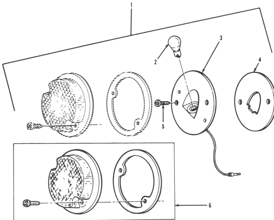
Figure 5-16 Rear-Side Marker Lamp
