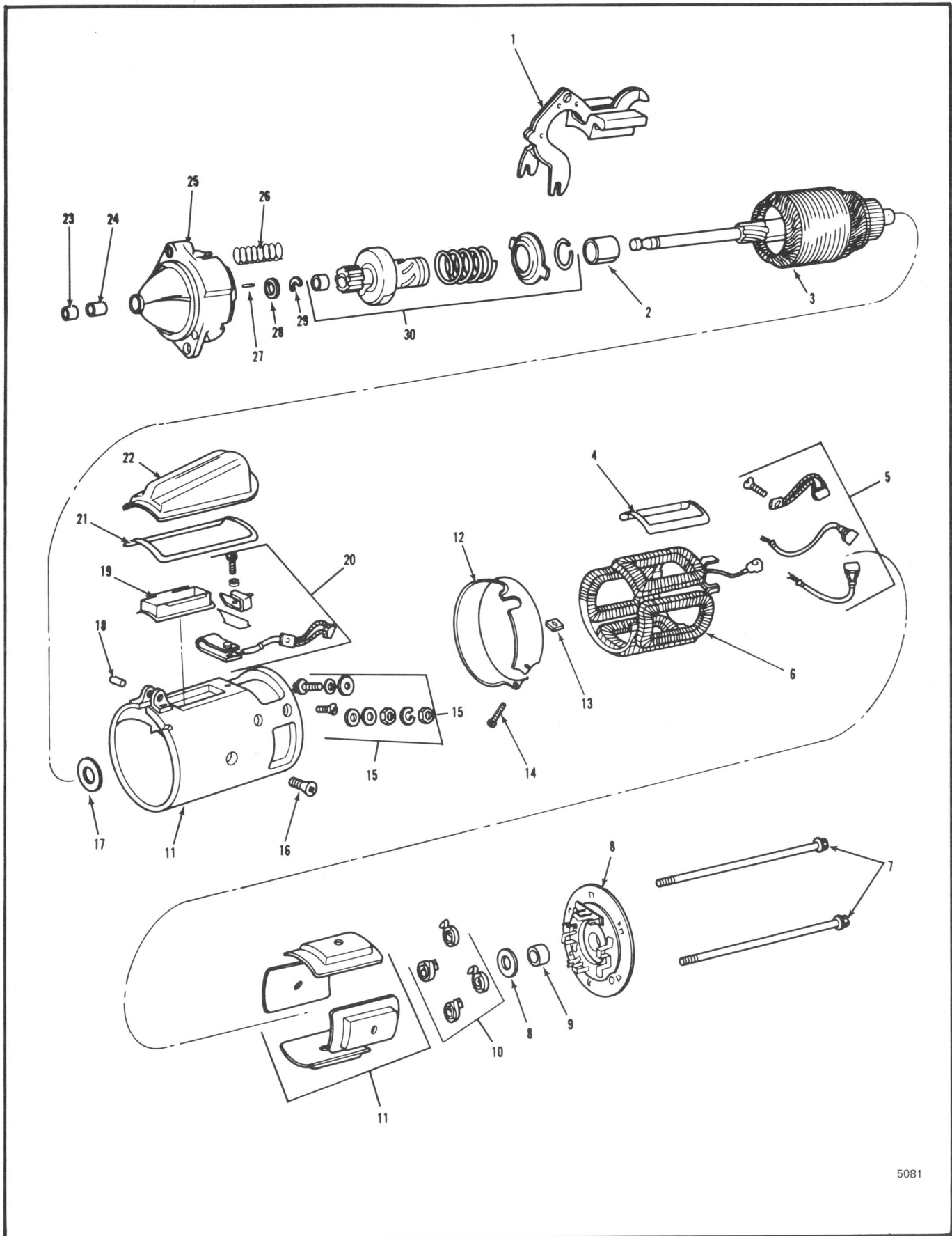
Figure 5-3 Starting Motor
