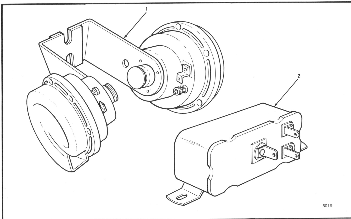
Figure 5-22 Horns
