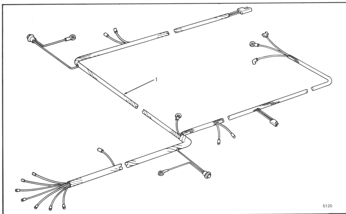
Figure 5-25 Body Wiring Harness
