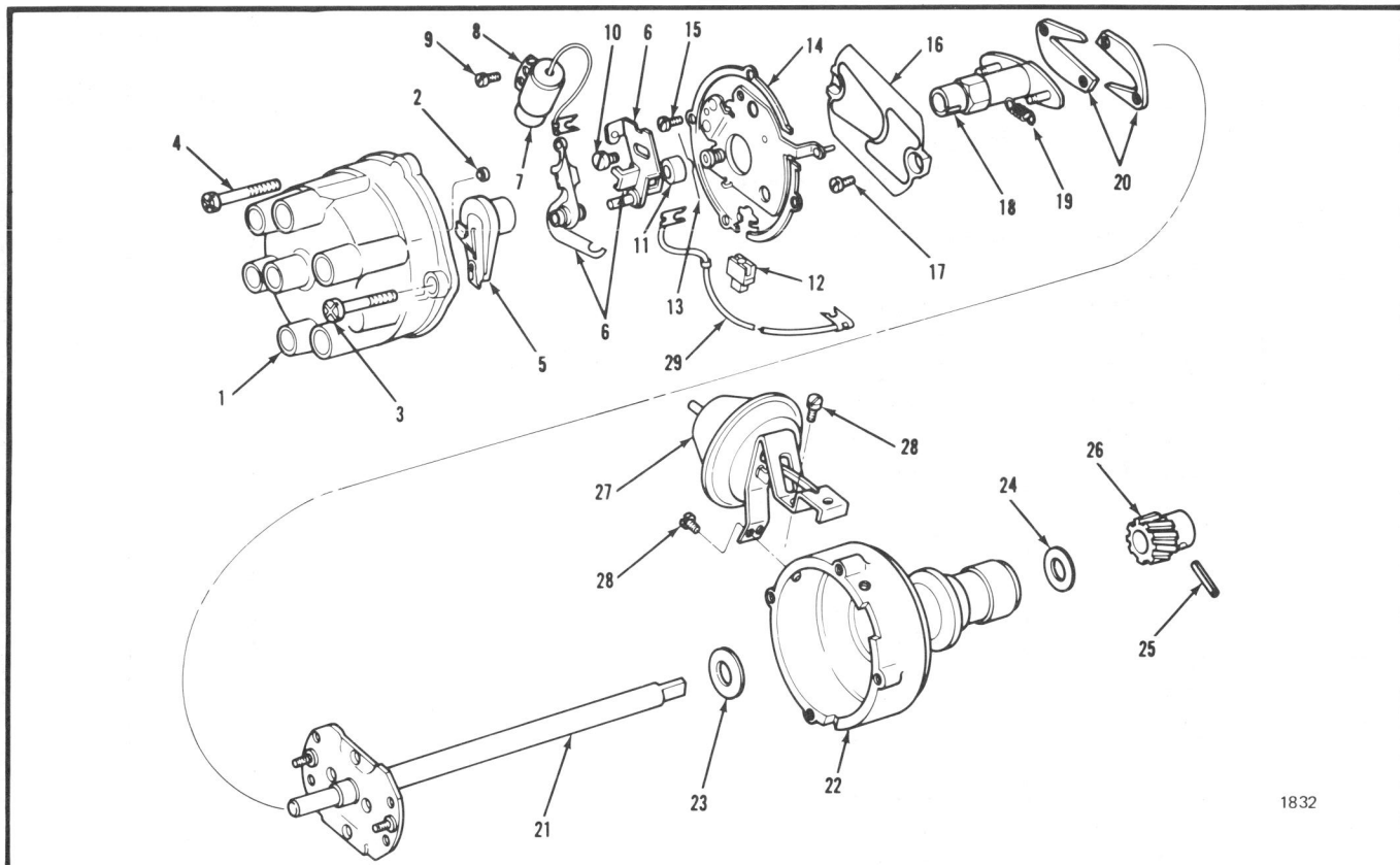
Figure 5-4 Distributor (A & B)
