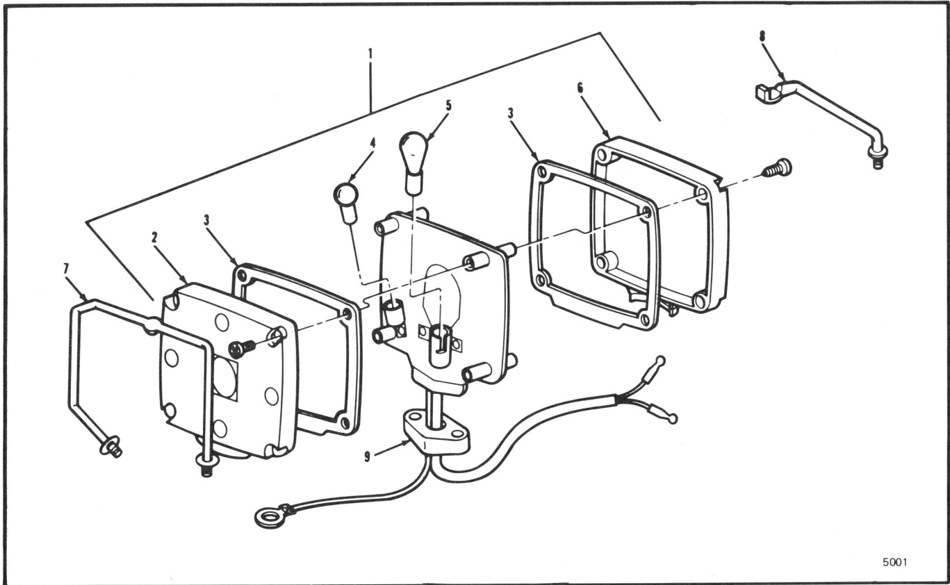
Figure 5-8 Front Signal Lamp
