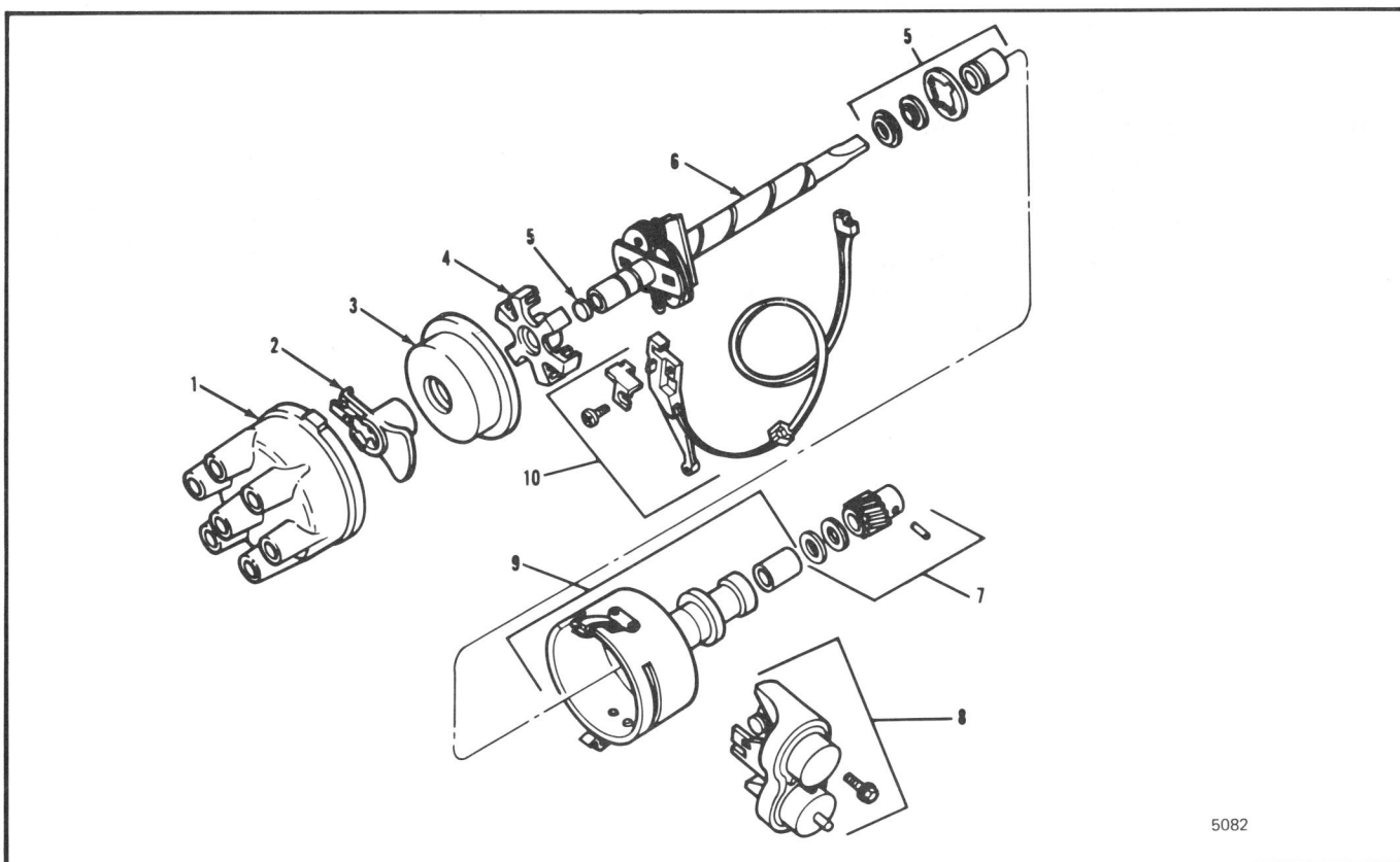
Figure 5-5 Distributor (C)
