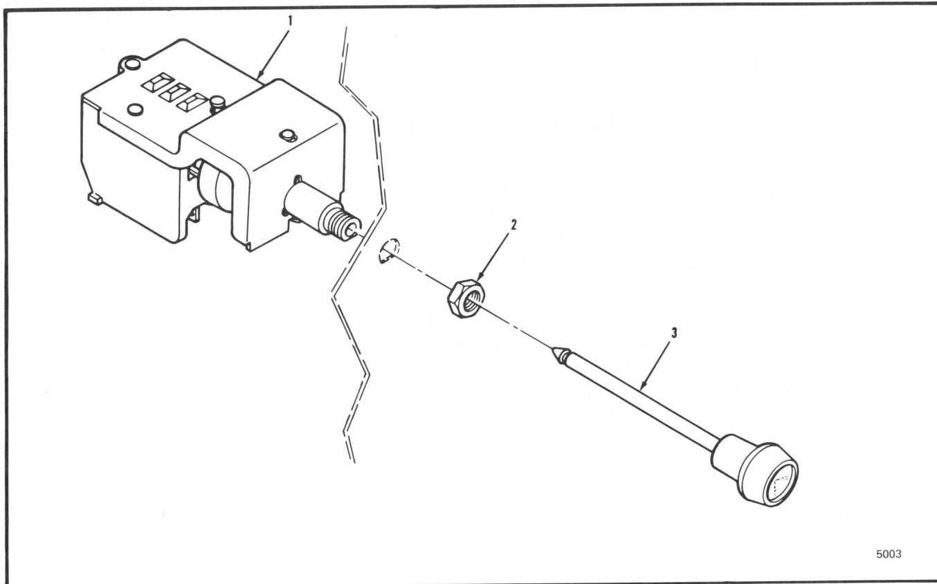
Figure 5-10 Main Light Switch
