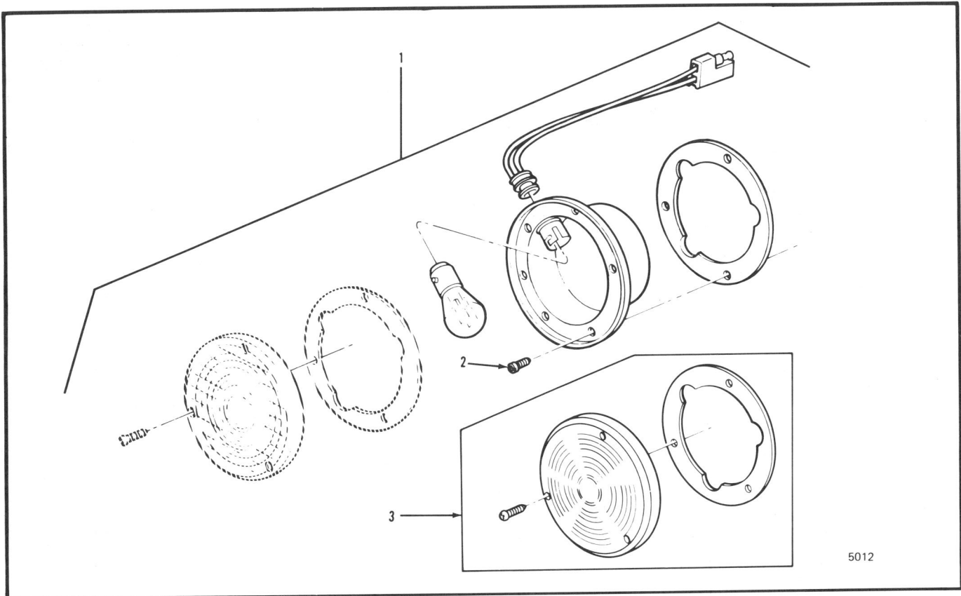
Figure 5-18 Tail, Stop and License Plate Lamps & Reflector
