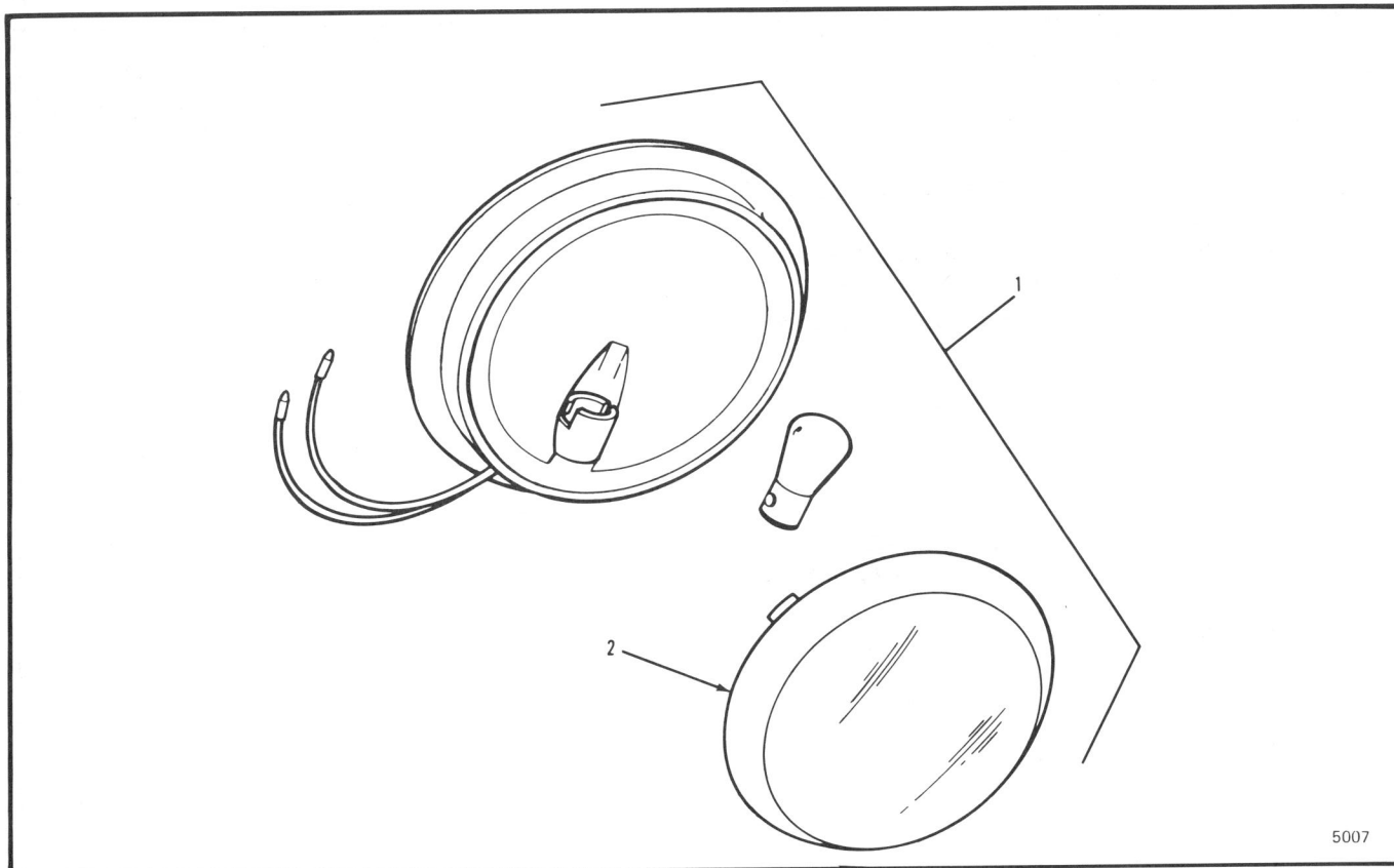
Figure 5-14 Dome Light
