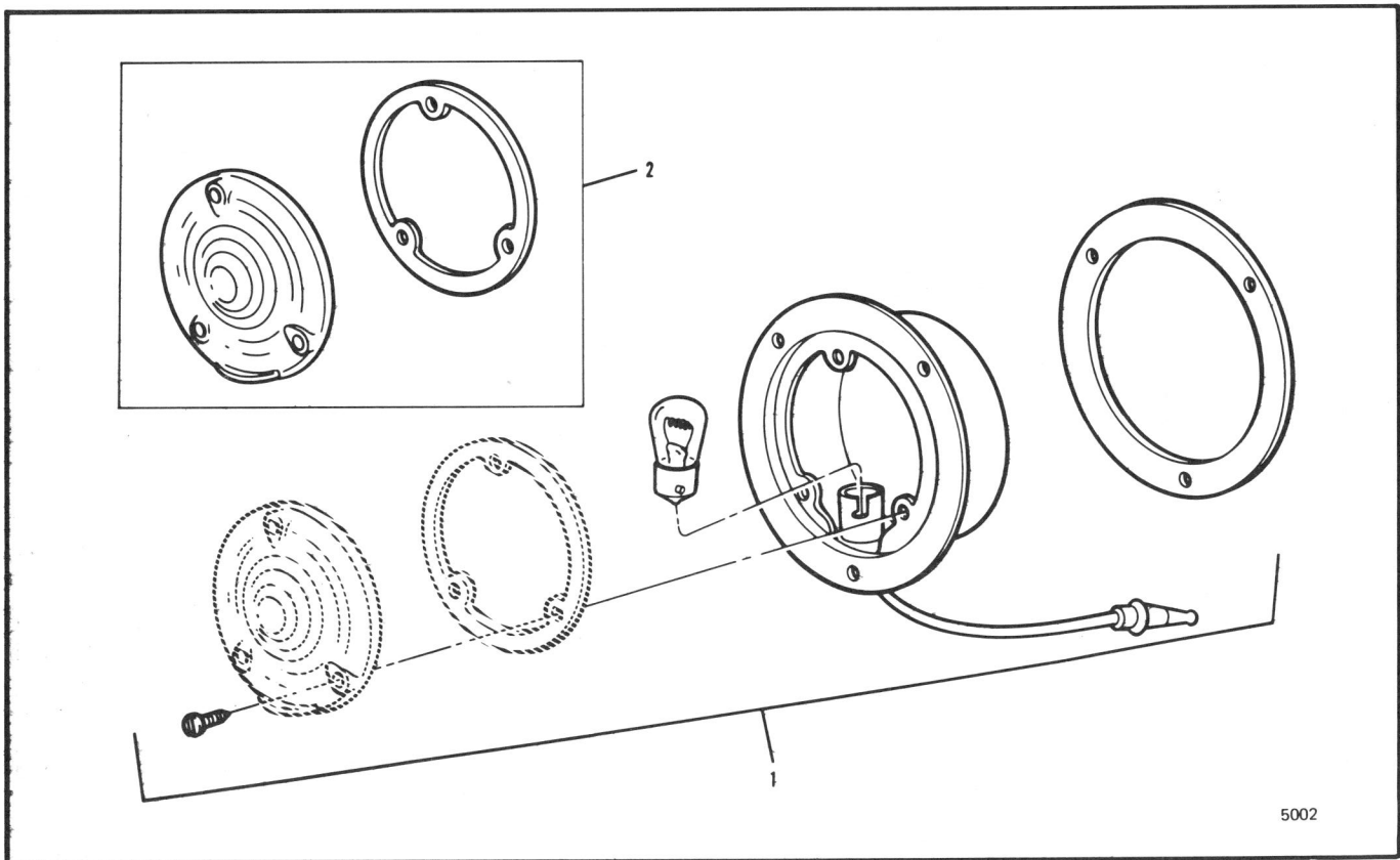
Figure 5-9 Rear Signal Lamp
