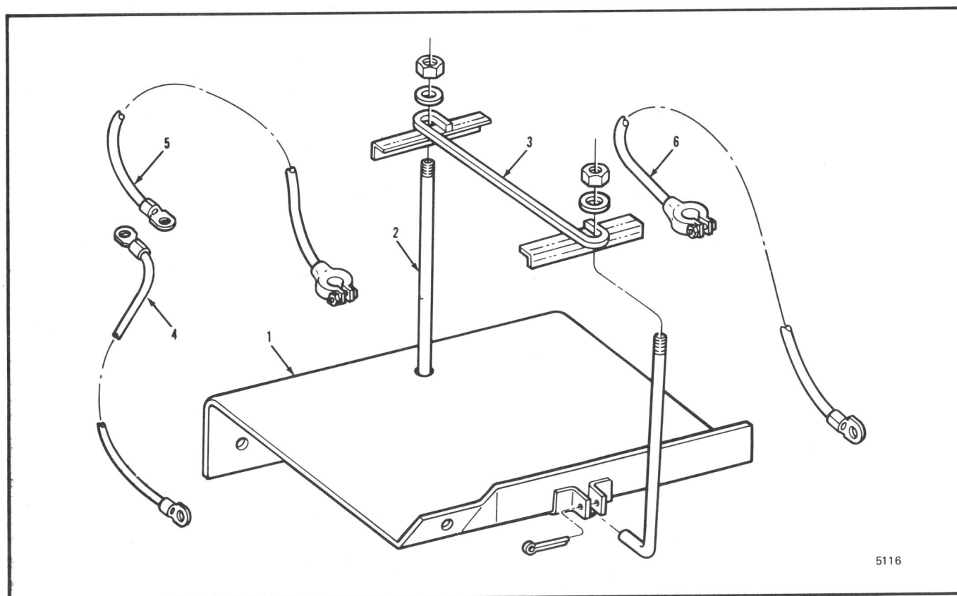
Figure 5-23 Battery Supports and Cables
