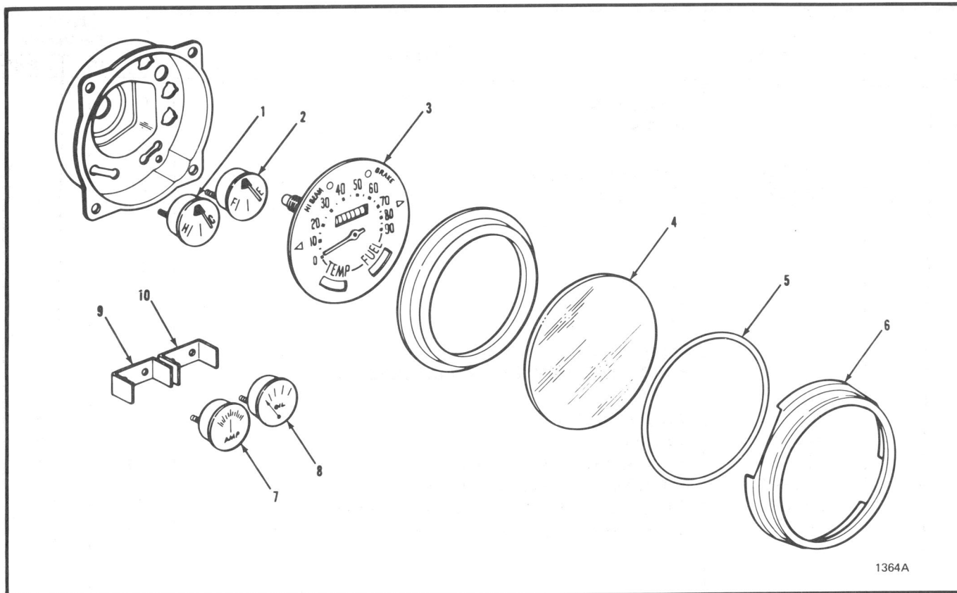
Figure 5-24 Instruments
