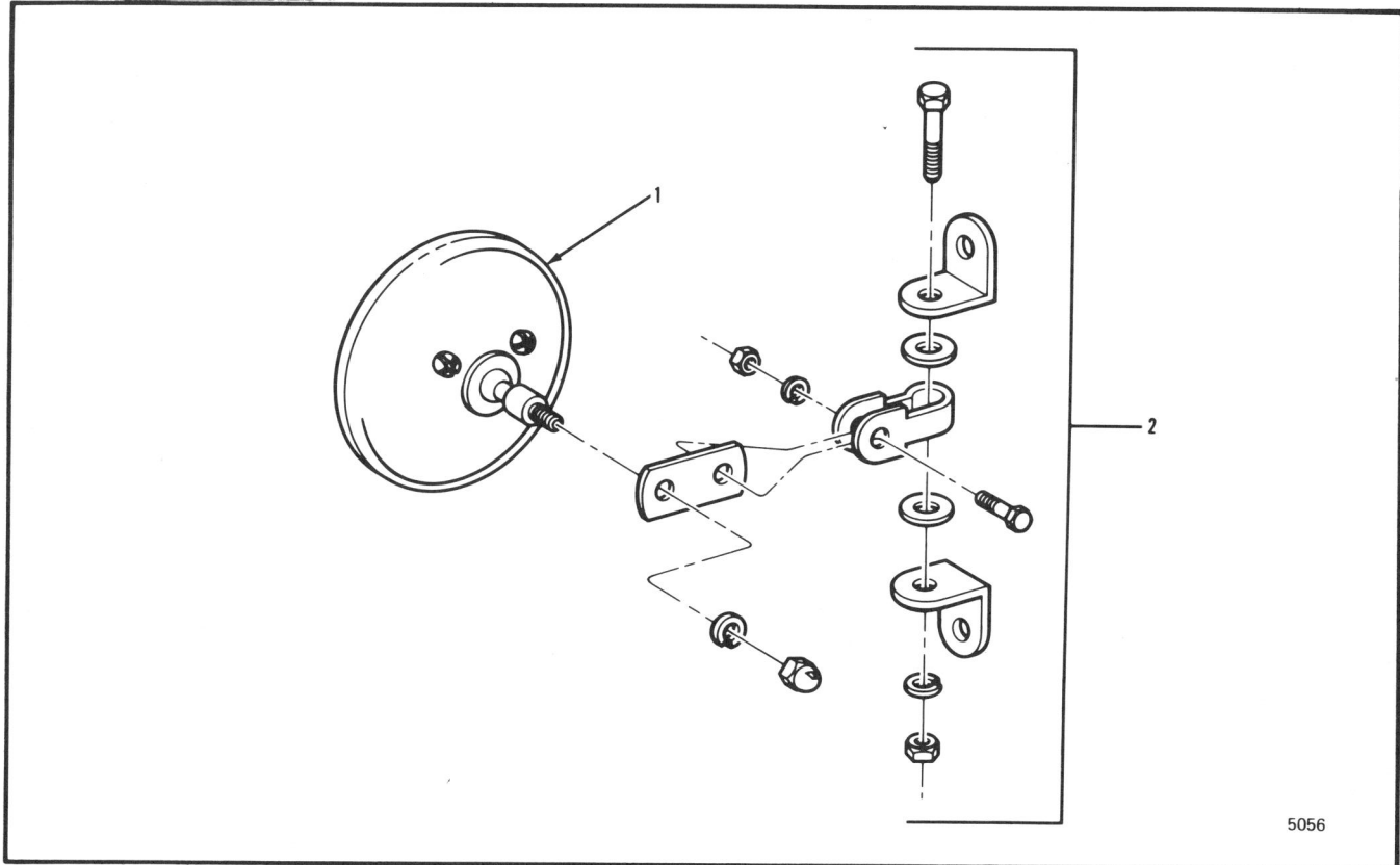
Figure 14-11 Driver's Side Mirror
