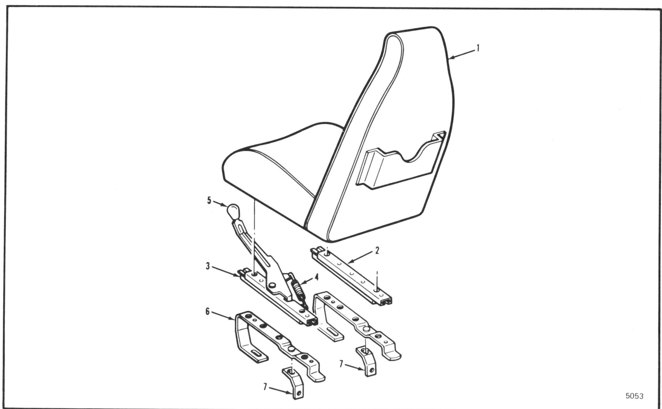
Figure 14-8 Seat
