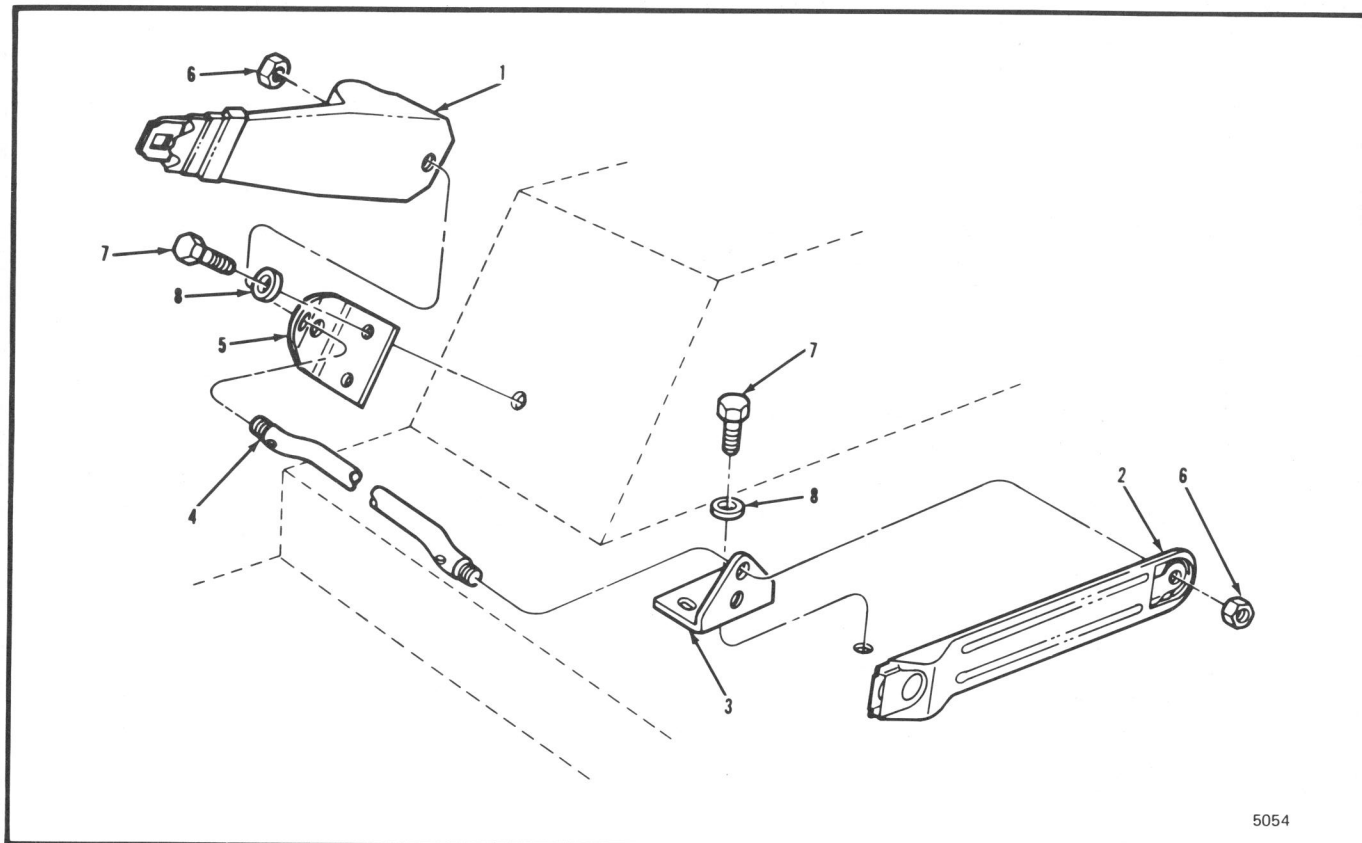
Figure 14-9 Seat Belts
