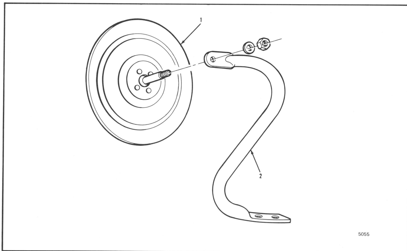
Figure 14-10 Convex Mirror, Fender Mount
