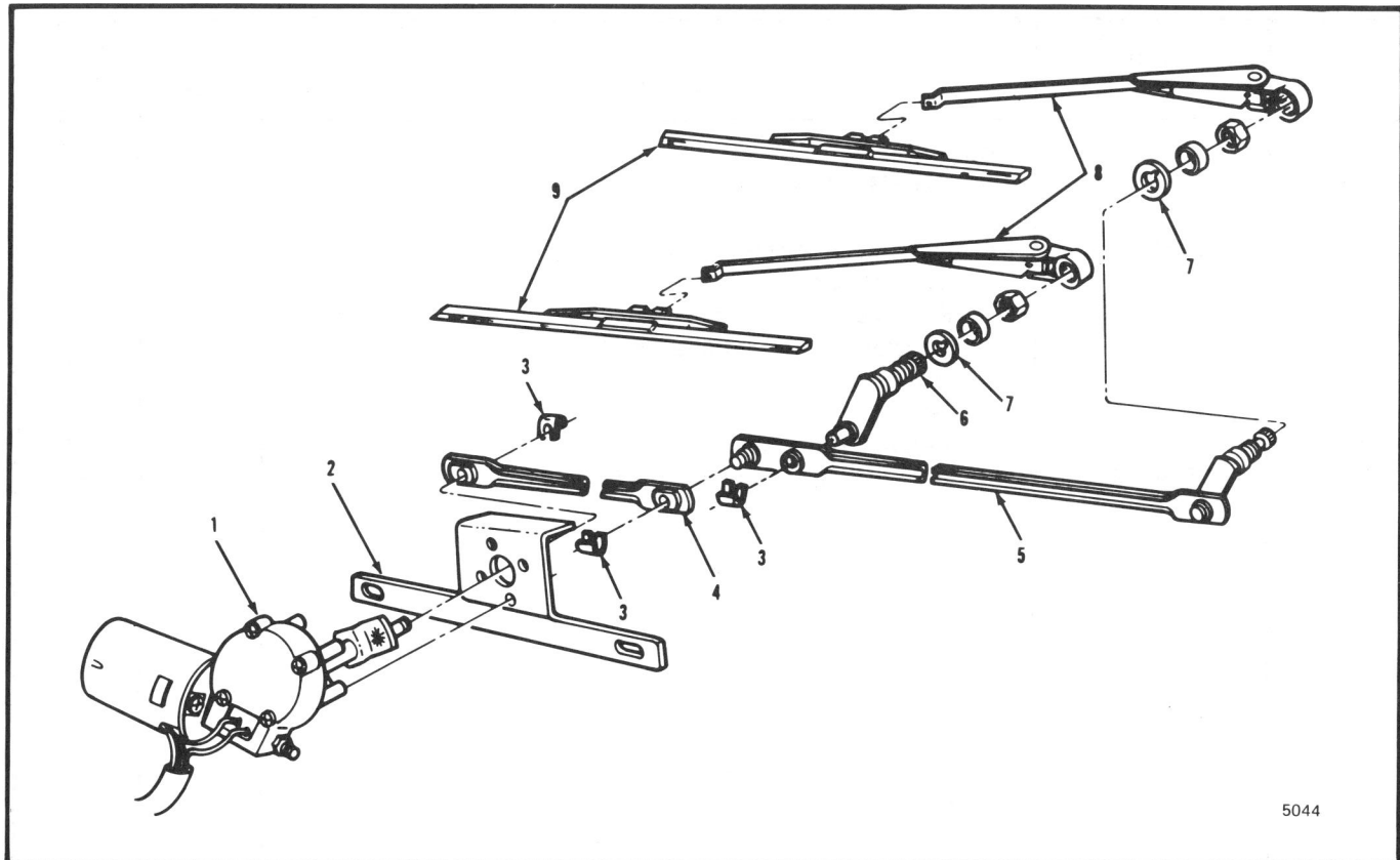
Figure 14-16 Windshield Wiper
