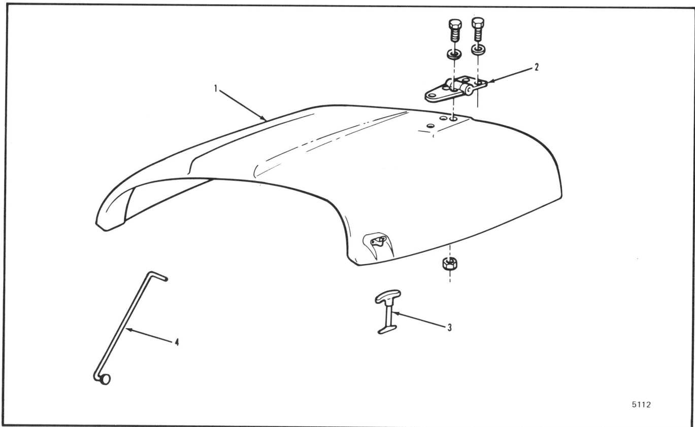
Figure 14-2 Hood
