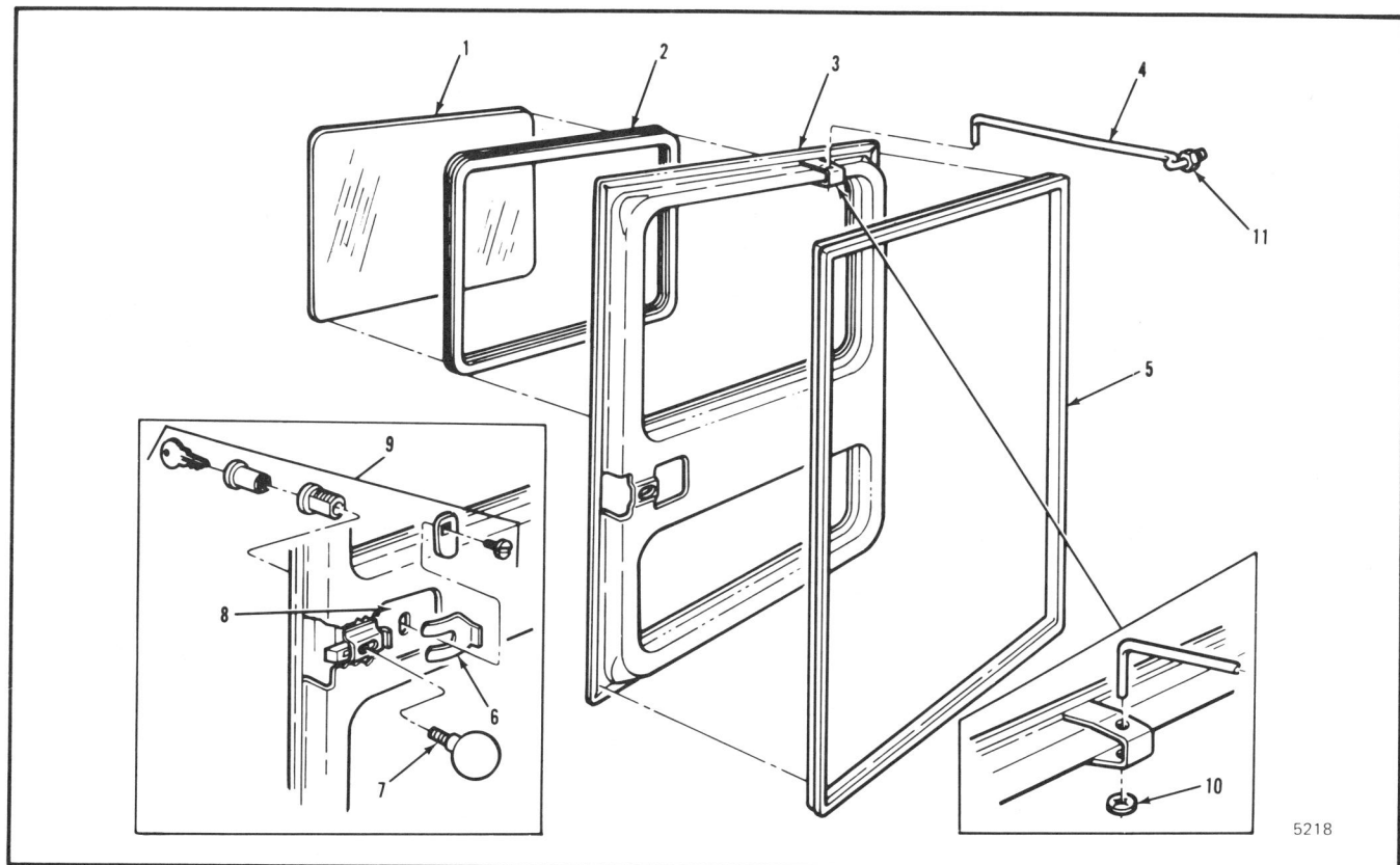
Figure 14-7 Rear Door
