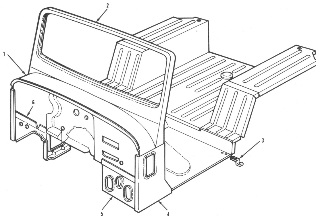
Figure 14-3 Body Front End and Underbody (Left Front View)
